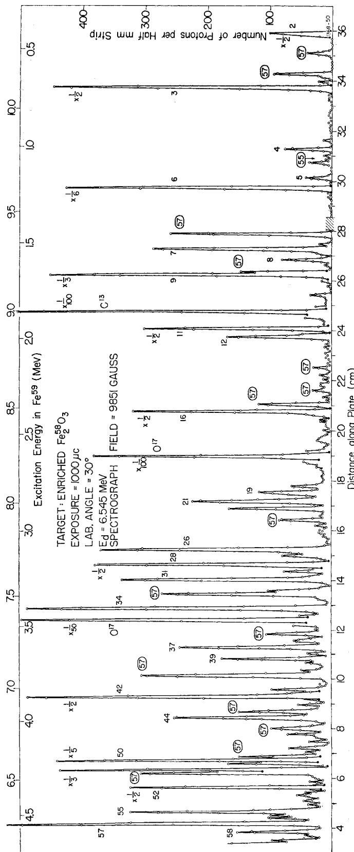
FIG. 12. Spectrum of protons from deuteron bombardment of a thin iron target enriched in Fe 58 (75.1%).
