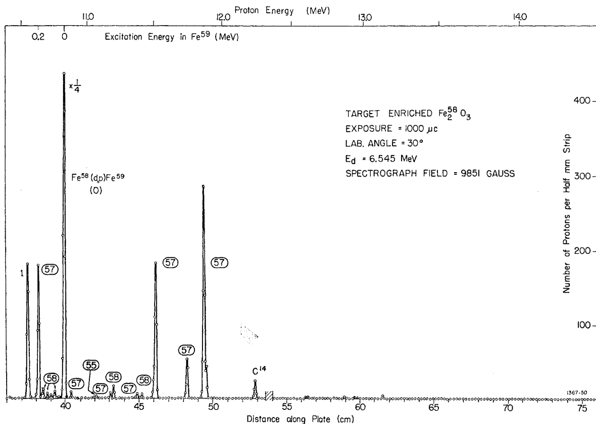
FIG. 8. Spectrum of protons from deuteron bombardment of a thin iron target enriched in \text{Fe}^{58} (75.1%).
