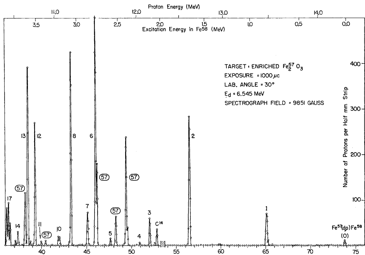
Fig. 7. Spectrum of protons from deuteron bombardment of a thin iron target enriched in \text{Fe}^{57} (84.1%).
